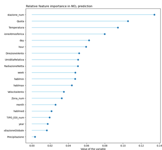
Figure 8 Distribution of residues (a), cumulative distribution of the same in absolute value (b) and relative feature importance in \text{NO}_2 prediction (c).
