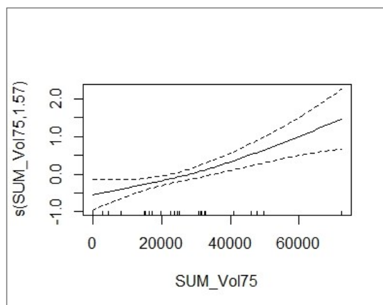
Fig. 17 - Toluene_winter_ex ante model: spline trend for the “sum of the volumes of the buildings in a buffer with a radius of 75 m” (k=5)
