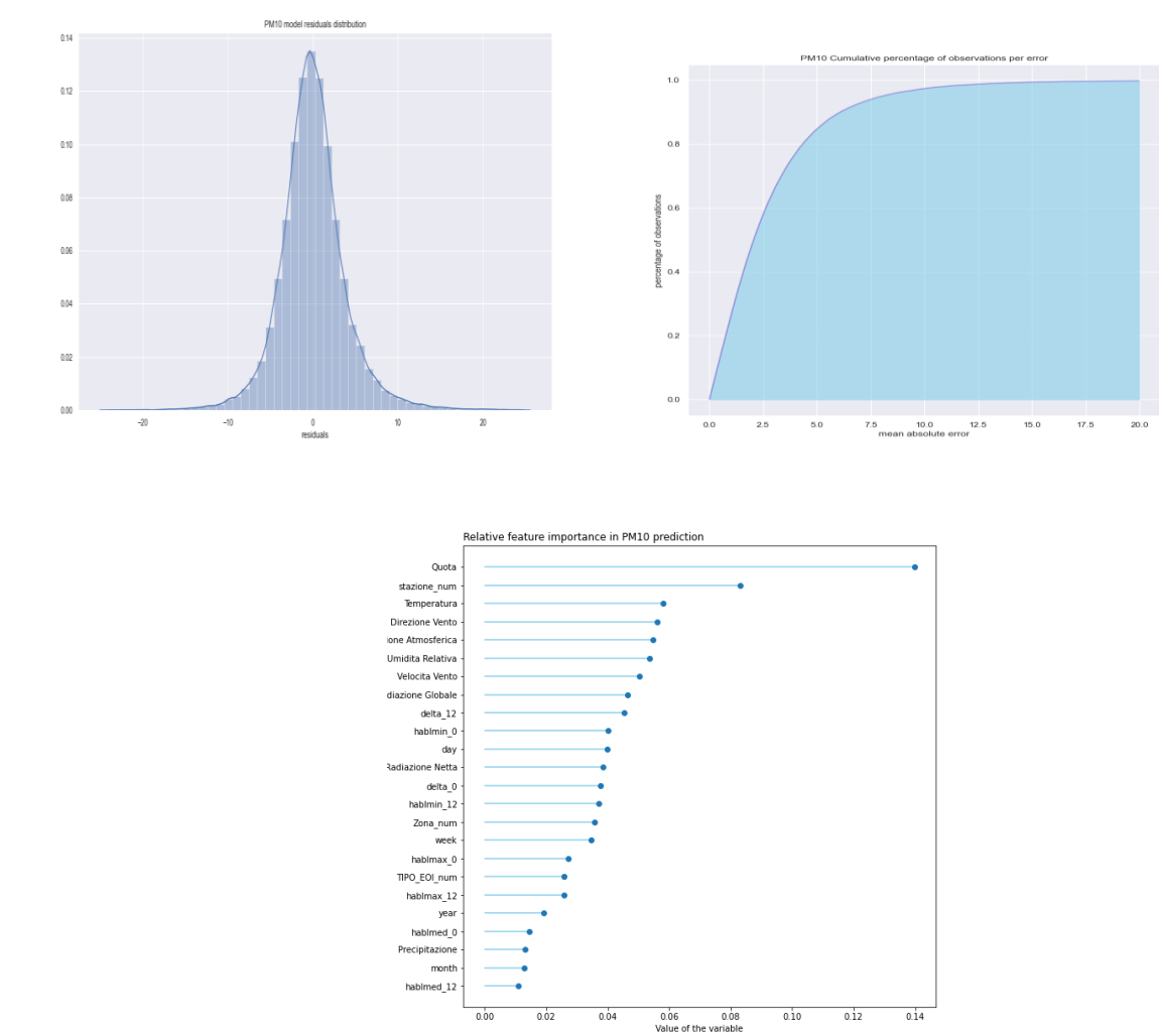
Figure 10 Distribution of residues (a), cumulative distribution of the same in absolute value (b) and relative feature importance in PM 10 prediction (c).
