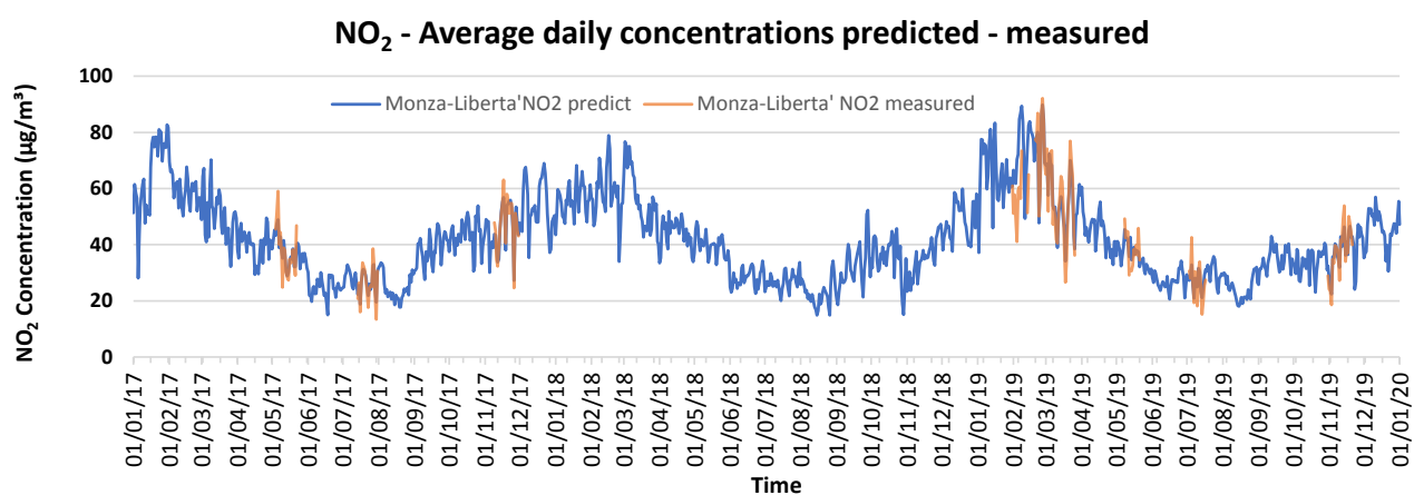
Figure 9. Comparison of the predicted and measured \text{NO}_2 daily averages.
